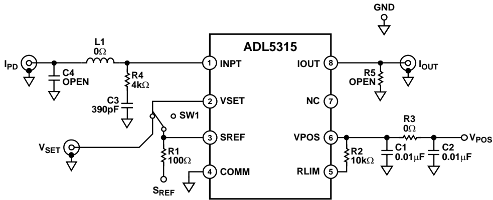
Figure 35. Evaluation Board Schematic (Rev. A)
