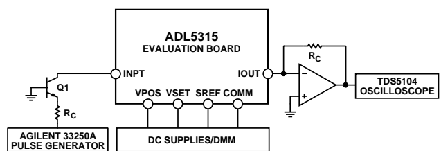
Figure 32. Configuration for Pulse Response of I_{INPT} to I_{OUT}
