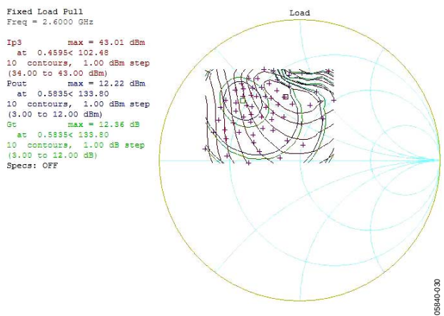
Figure 30. Load-Pull Contours, 2600 MHz
