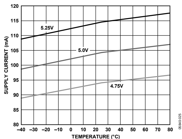
Figure 25. Supply Current vs. Supply Voltage and Temperature (Using 880 MHz Matching Components)
