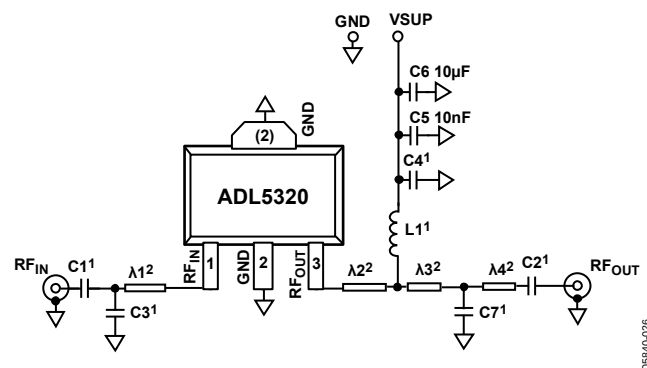
Figure 26. Basic Connections
