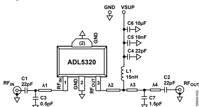
Figure 32. Evaluation Board, 1805 MHz to 2170 MHz
