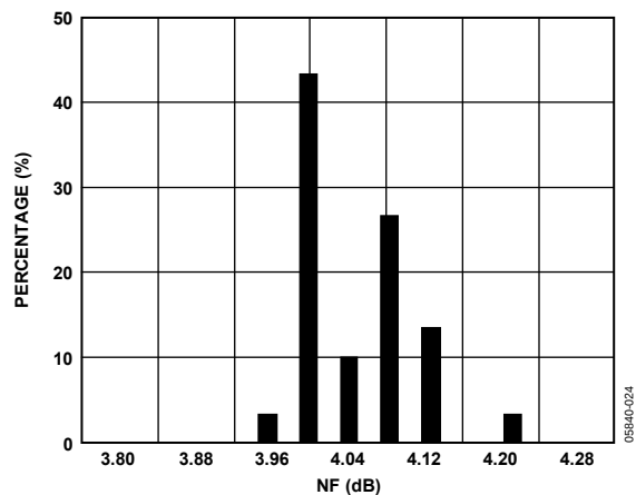
Figure 24. Noise Figure Distribution at 880 MHz
