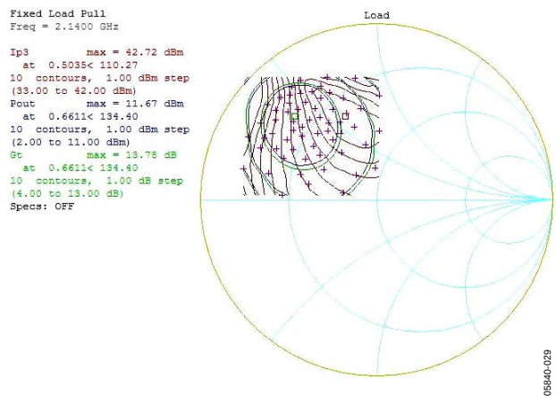
Figure 29. Load-Pull Contours, 2140 MHz
