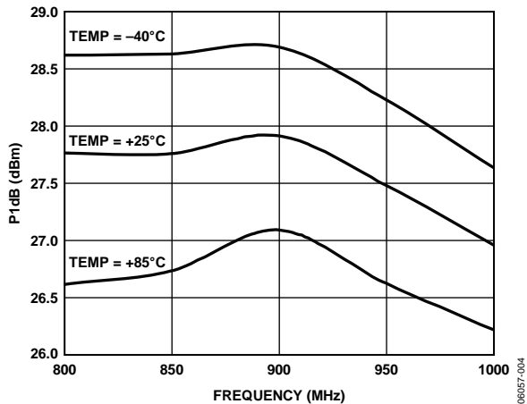
Figure 4. P1\text{ dB} vs. Frequency, V_{CC} = 5\text{ V} , T_A = -40^\circ\text{C} , +25^\circ\text{C} , and +85^\circ\text{C}
