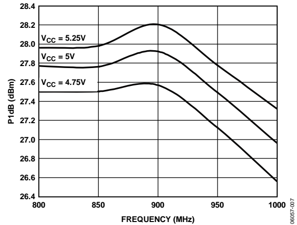
Figure 7. P1\text{ dB} vs. Frequency, V_{CC} = 4.75\text{ V} , 5\text{ V} , and 5.25\text{ V} , T_A = 25^\circ\text{C}
