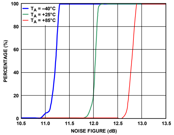
Figure 25. Noise Figure Distributions
