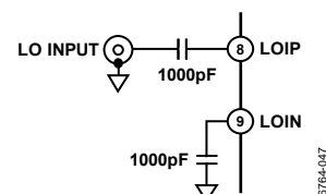
Figure 46. Single-Ended LO Drive
