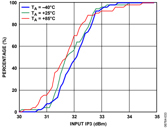
Figure 33. IIP3 Distributions
