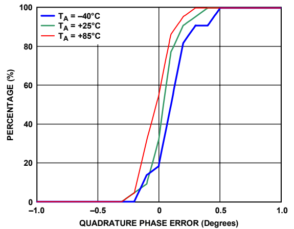
Figure 38. I/Q Quadrature Error Distributions
