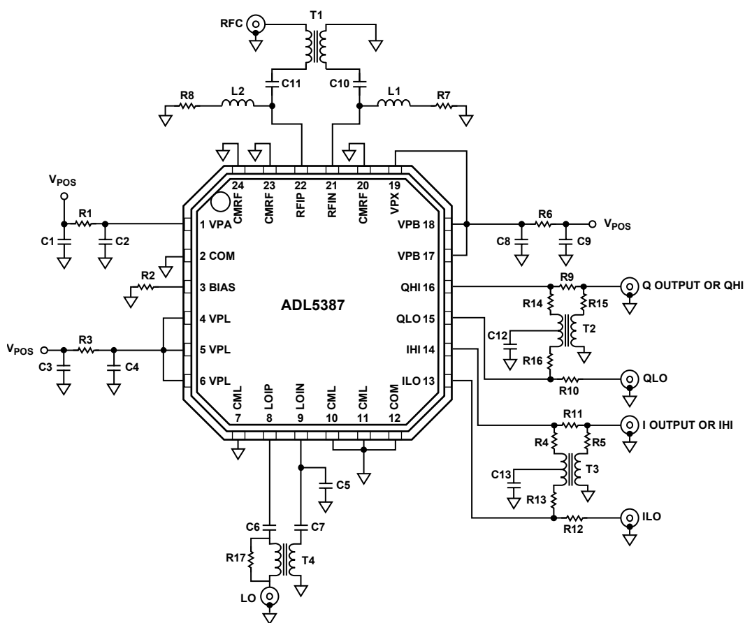
Figure 63. Evaluation Board Schematic
