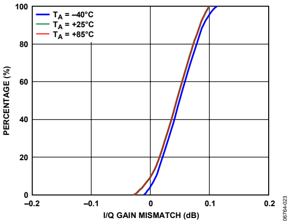
Figure 23. I/Q Gain Mismatch Distributions
