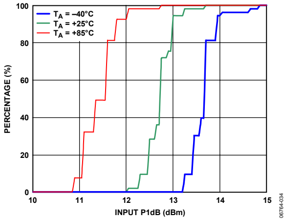
Figure 34. IP1dB Distributions
