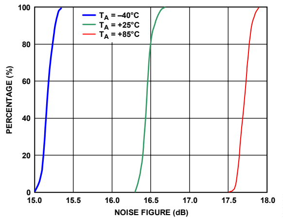
Figure 43. Noise Figure Distributions
