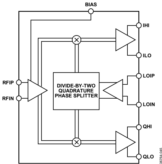
Figure 45. Block Diagram
