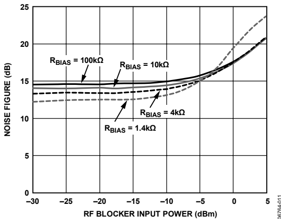
Figure 11. Noise Figure vs. Input Blocker Level, f_{RF} = 900 MHz (RF Blocker 5 MHz Offset)
