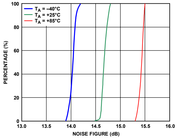
Figure 37. Noise Figure Distributions
