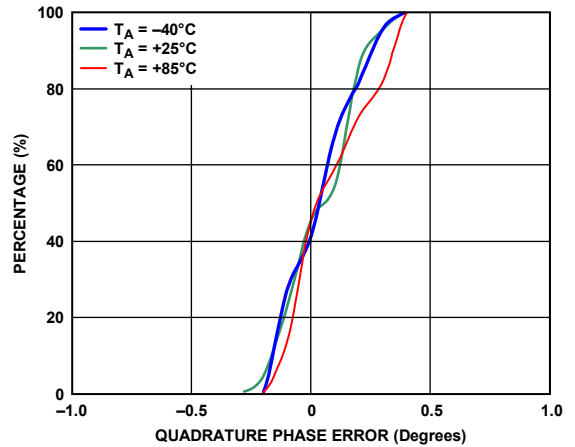
Figure 26. I/Q Quadrature Error Distributions
