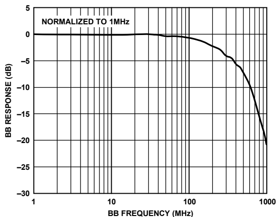
Figure 6. Normalized I/Q Baseband Frequency Response
