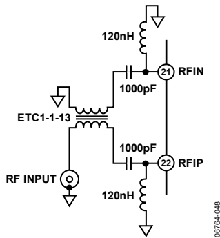
Figure 48. RF Input
