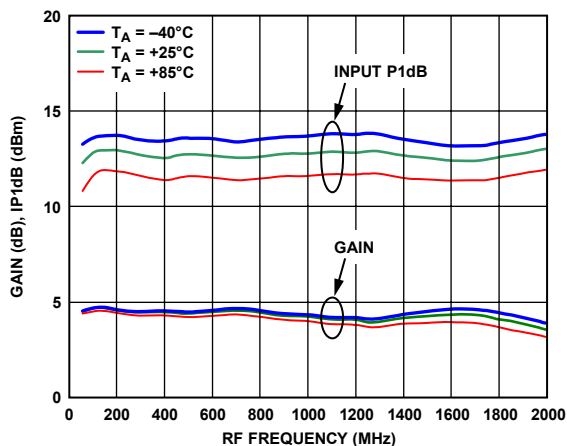
Figure 3. Conversion Gain and Input 1 dB Compression Point (IP1dB) vs. RF Frequency
