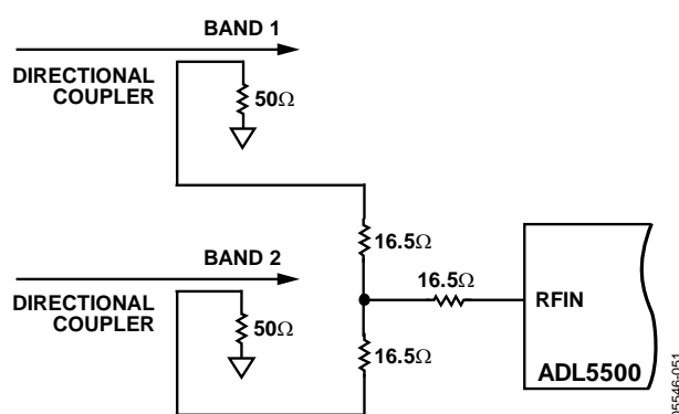
Figure 37. Combining Multiple RF Input Signals
