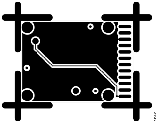
Figure 50. Layout of Circuit Side (WLCSP)
