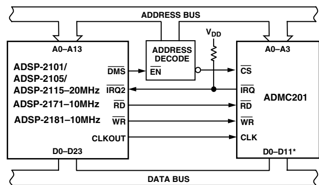
Figure 11. ADI Digital Signal Processor/Microcomputer
