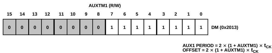
Figure 23. Configuration of AUX Registers
