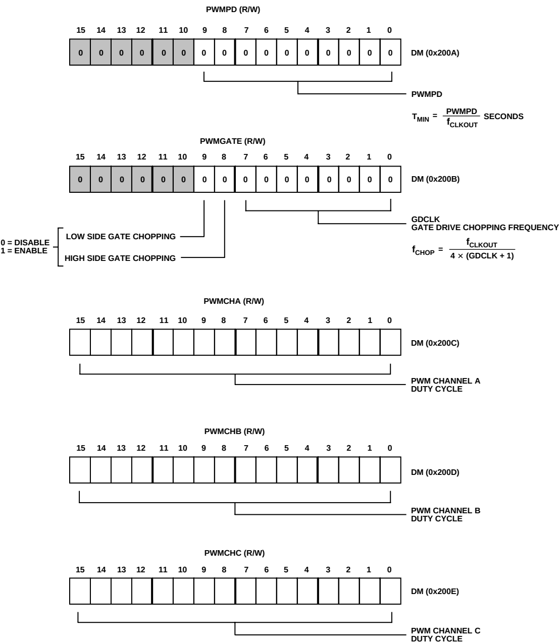
Figure 20. Configuration of Additional PWM Registers
