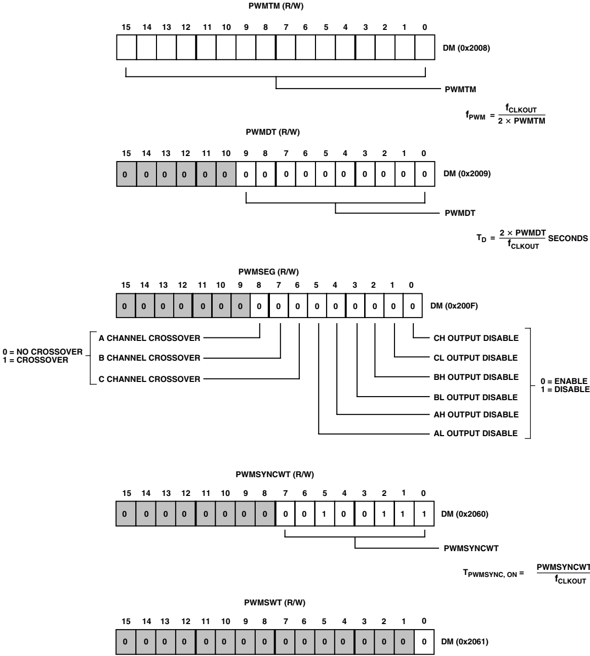
Figure 20. Configuration of PWM Registers
