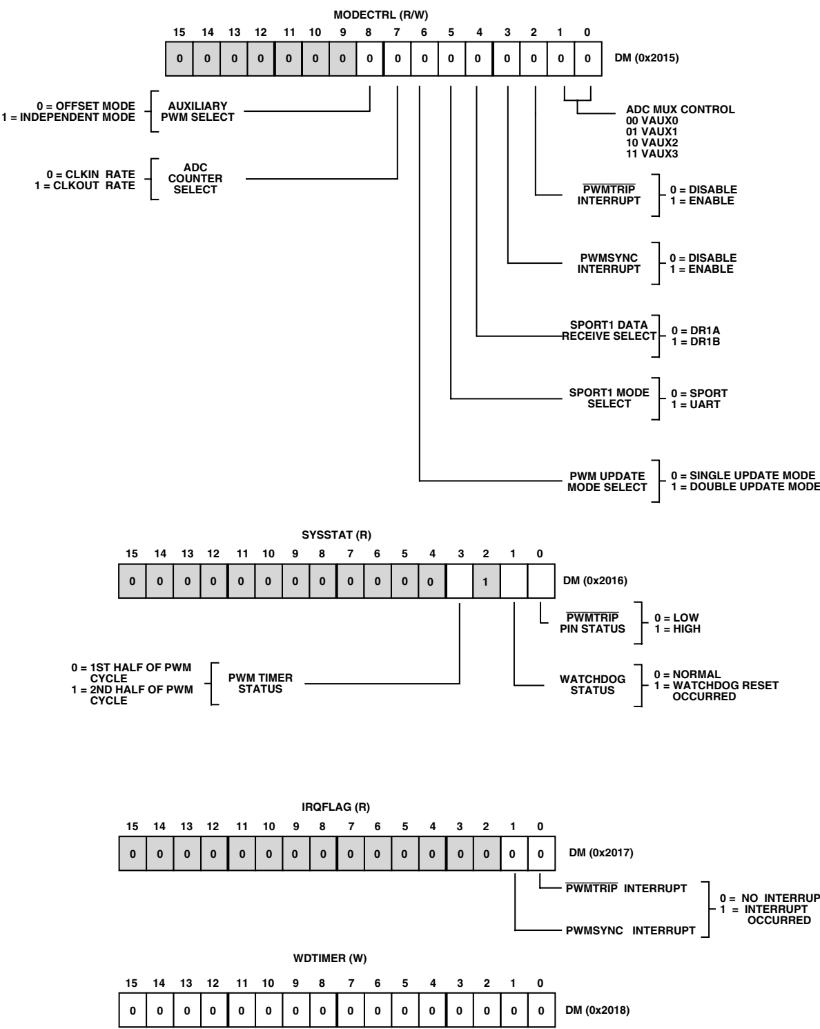
Figure 26. Configuration of Status Registers
