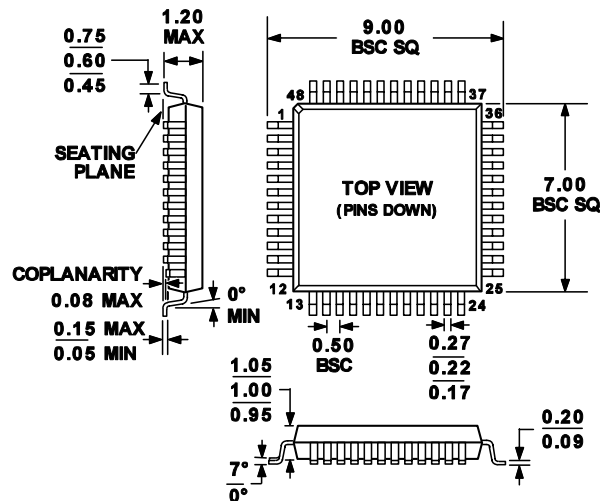
Figure 50. 48-Lead 7×7 TQFP Package (SU-48)
