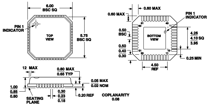
Figure 49. 40-Lead 6×6 Chip Scale Package (CP-40)
