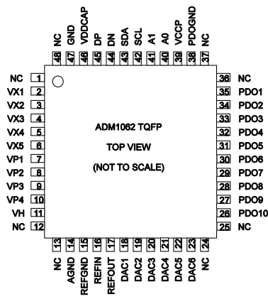
Figure 4. TQFP Pin Configuration
