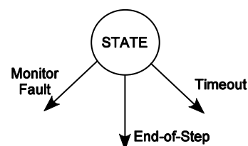
Figure 27. State Cell
