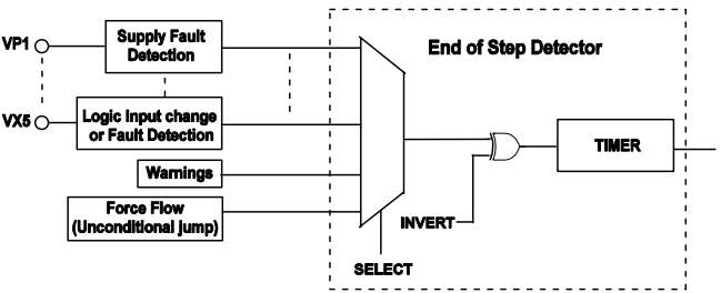
Figure 30. End-of-Step Detector
