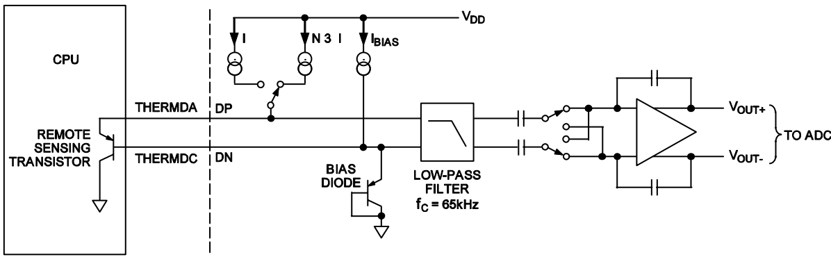
Figure 33. Signal Conditioning for Remote Diode temperature Sensors
