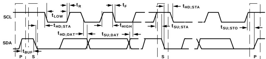
Figure 28. Serial Bus Timing Diagram
