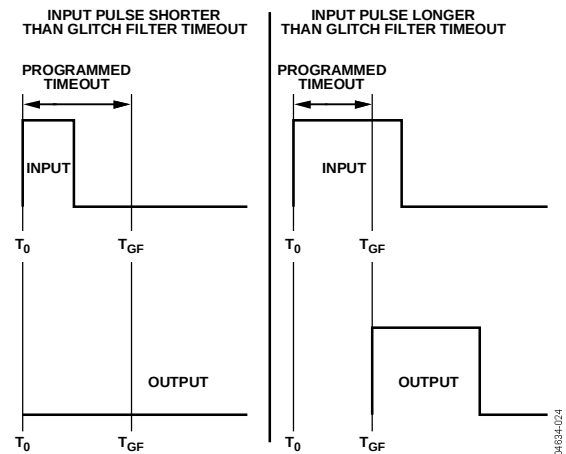
Figure 17. Input Glitch Filter Function
