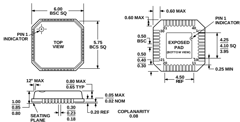
Figure 38. 40-Lead Lead Frame Chip Scale Package [LFCSFP] (CP-40)
