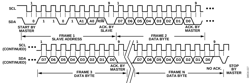
Figure 27. General SMBus Read Timing Diagram
