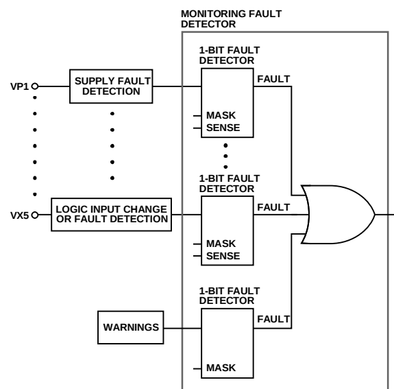
Figure 23. Monitoring Fault Detector Block Diagram
