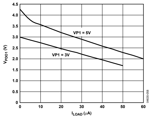
Figure 13. V_{PDO1} (Weak Pull-Up to V_P ) vs. I_{LOAD}
