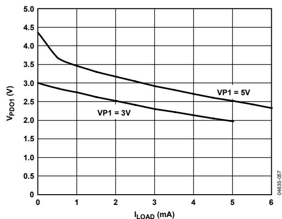
Figure 12. V_{PDO1} (Strong Pull-Up to V_P ) vs. I_{LOAD}
