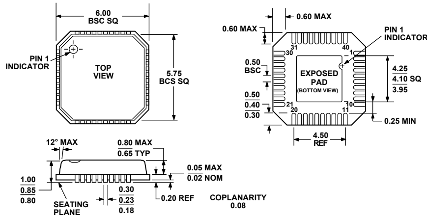
Figure 42. 40-Lead Lead Frame Chip Scale Package [LFCSP_VQ] 6 mm x 6 mm Body, Very Thin Quad (CP-40)
