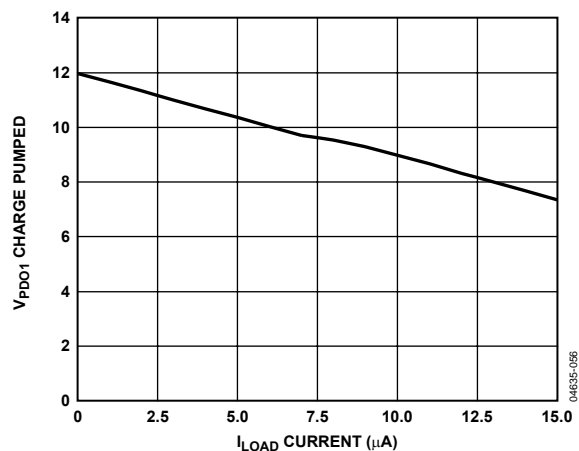
Figure 11. V_{PDO1} (FET Drive Mode) vs. I_{LOAD}
