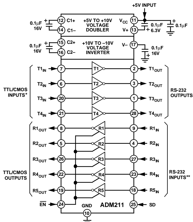
Figure 12. ADM211 Typical Operating Circuit
