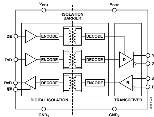
Figure 25. Digital Isolation and Transceiver Sections
