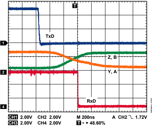
Figure 8. Driver/Receiver Propagation Delay, High to Low ( R_L = 54\ \Omega , C_{L1} = C_{L2} = 100\ \text{pF} )
