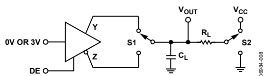
Figure 18. Driver Enable/Disable
