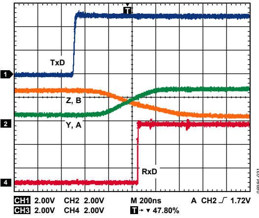
Figure 7. Driver/Receiver Propagation Delay, Low to High ( R_L = 54\ \Omega , C_{L1} = C_{L2} = 100\ \text{pF} )
