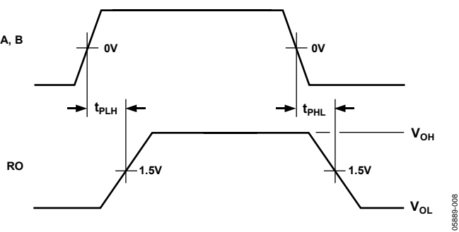
Figure 9. Receiver Propagation Delay
