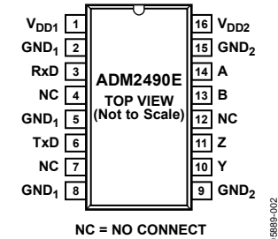
Figure 2. ADM2490E Pin Configuration
