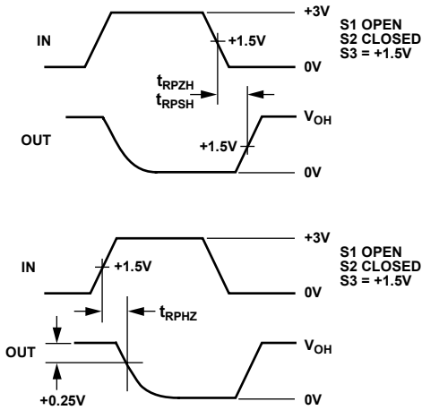
Figure 15. Receiver Enable and Disable Times
