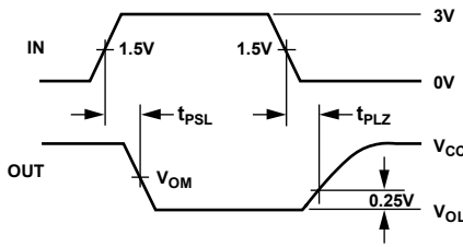
Figure 13. Driver Enable and Disable Times ( t_{PLZ} , t_{PSL} , t_{PLZ} )
