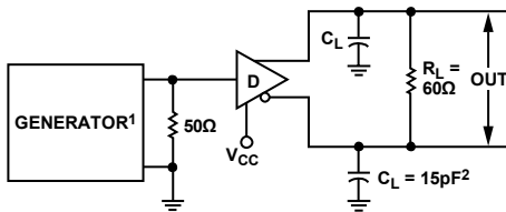
1 PPR = 250kHz, 50% DUTY CYCLE, t_r \leq 6.0\text{ns} , Z_0 = 50\Omega . 2 C_L INCLUDES PROBE AND STRAY CAPACITANCE.
