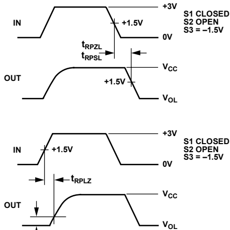
Figure 15. Receiver Enable and Disable Times
