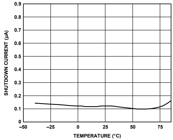
Figure 25. Shutdown Current vs. Temperature
