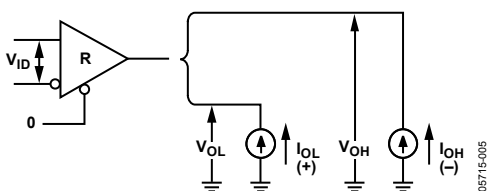
Figure 5. Receiver V_{OH} and V_{OL}
