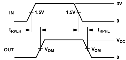
Figure 16. Receiver Propagation Delay
