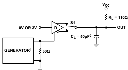
Figure 8. Driver Enable and Disable Times ( t_{pZH} , t_{psH} , t_{pLH} )
