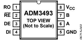
Figure 2. Pin Configuration
