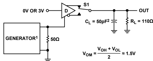
Figure 8. Driver Enable and Disable Times ( t_{pZH} , t_{psH} , t_{pLH} )
