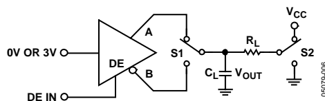
Figure 6. Driver Enable/Disable
