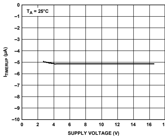
Figure 14. I TIMERUP (in Initial Cycle) vs. Supply Voltage
