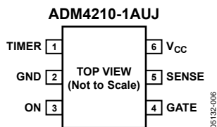
Figure 3. Pin Configuration, 1AUJ Model
