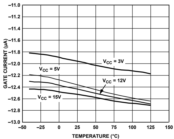
Figure 11. GATE Current (up) vs. Temperature
