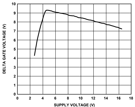
Figure 12. Delta GATE Voltage vs. Supply Voltage
