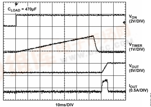
Figure 2. Start-Up Sequence
