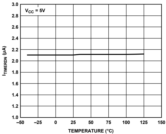
Figure 19. I_{TIMERDN} (in Cool-Off Cycle) vs. Temperature
