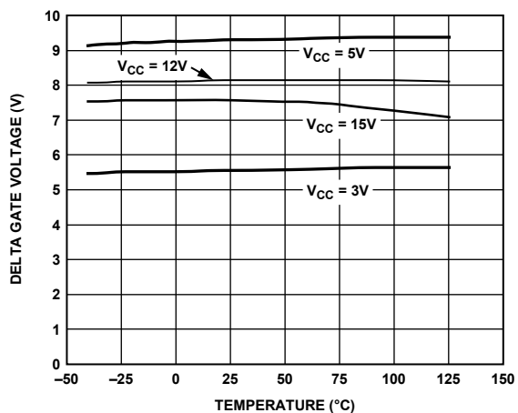
Figure 13. Delta GATE Voltage vs. Temperature
