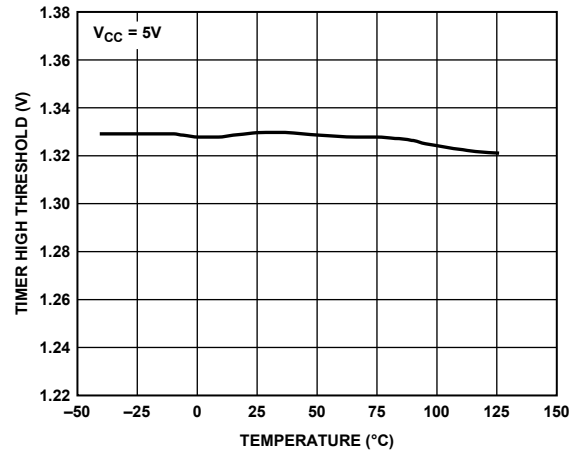
Figure 21. TIMER High Threshold vs. Temperature
