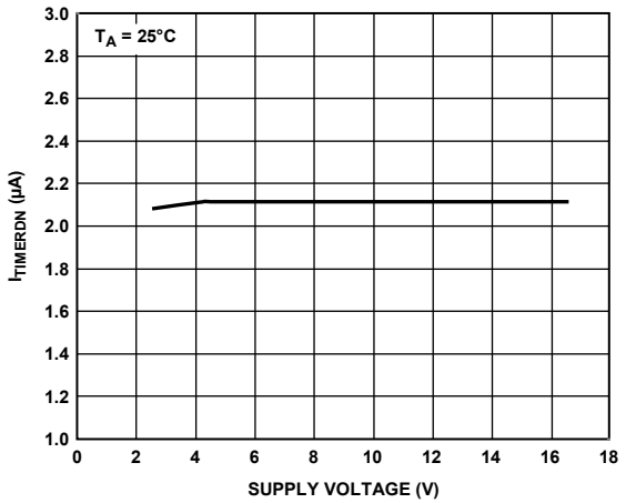
Figure 18. I_{TIMERDN} (in Cool-Off Cycle) vs. Supply Voltage
