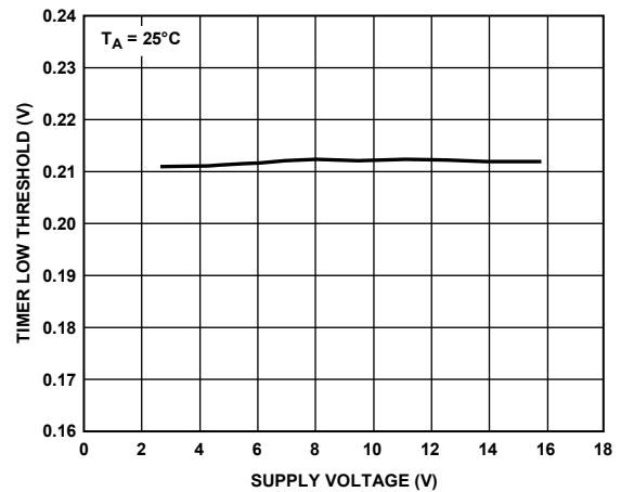
Figure 22. TIMER Low Threshold vs. Supply Voltage
