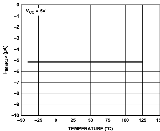
Figure 15. I TIMERUP (in Initial Cycle) vs. Temperature
