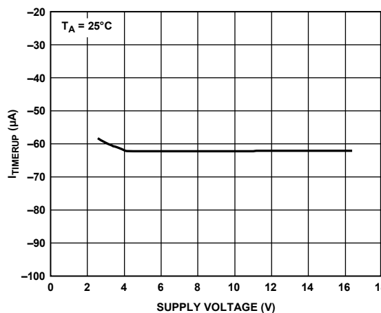
Figure 16. I TIMERUP (During Cct Breaker Delay) vs. Supply Voltage
