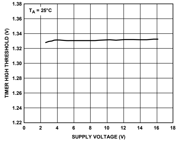
Figure 20. TIMER High Threshold vs. Supply Voltage
