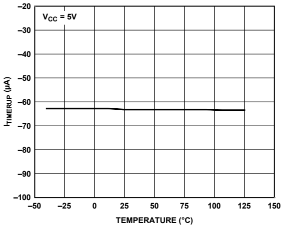
Figure 17. I_{TIMERUP} (During Cct Breaker Delay) vs. Temperature
