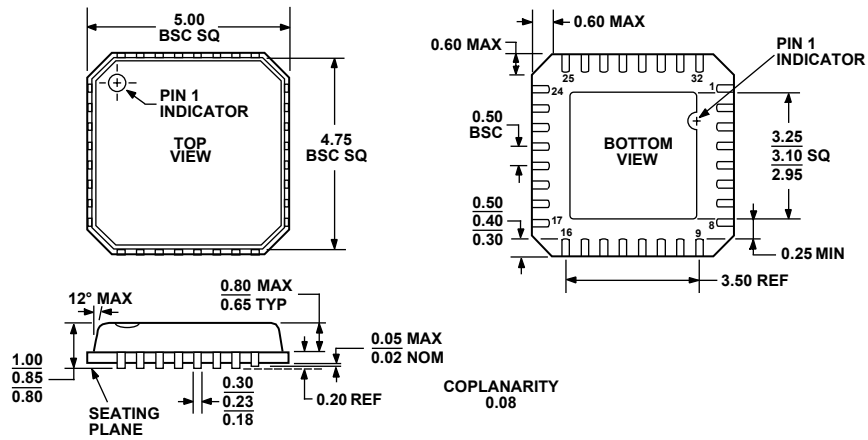
Figure 29. 32-Lead Frame Chip Scale Package [LFCSP] (CP-32)
