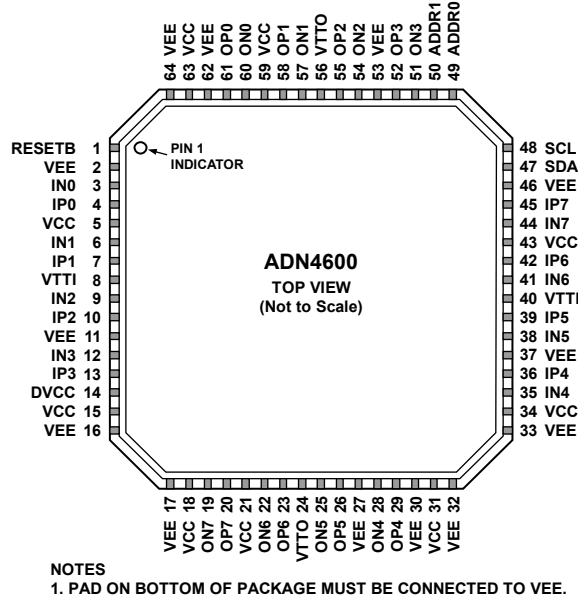
Figure 3. Pin Configuration
