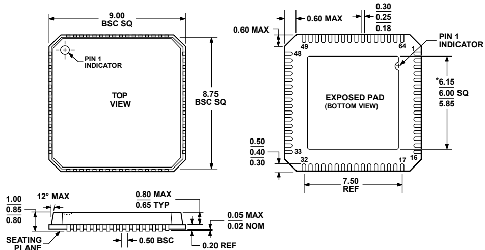
Figure 33. 64-Lead Lead Frame Chip Scale Package [LFCSP_VQ] 9 mm × 9 mm Body, Very Thin Quad (CP-64-2)
