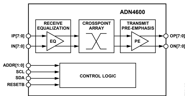
Figure 27. Simplified Functional Block Diagram
