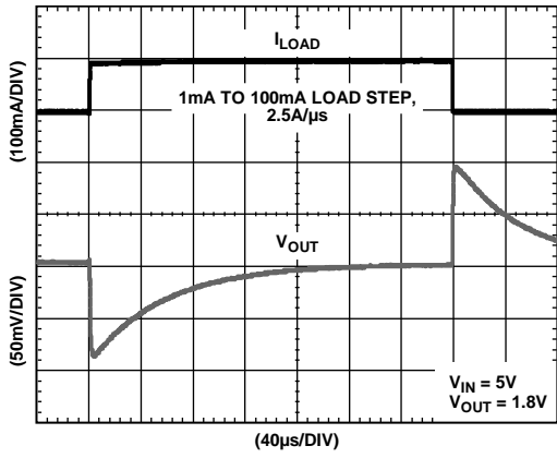
Figure 23. Load Transient Response, C_{IN} and C_{OUT} = 1\ \mu\text{F}
