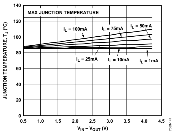
Figure 47. WLCSOP, T_B = 85^\circ\text{C}
