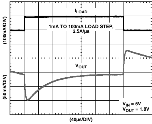
Figure 24. Load Transient Response, C_{IN} and C_{OUT} = 4.7\ \mu\text{F}
