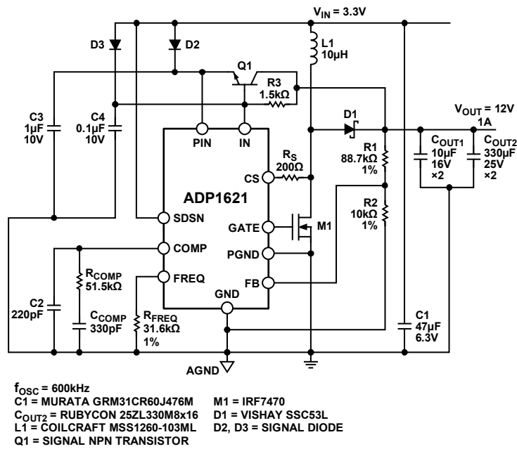
Figure 35. Bootstrapped Application Circuit for V_{OUT} > 5.5\text{ V}
