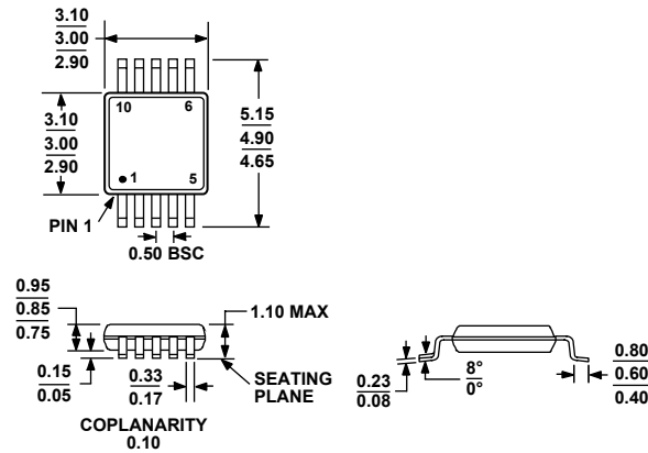
Figure 43. 10-Lead Mini Small Outline Package [MSOP] (RM-10) Dimensions shown in millimeters
