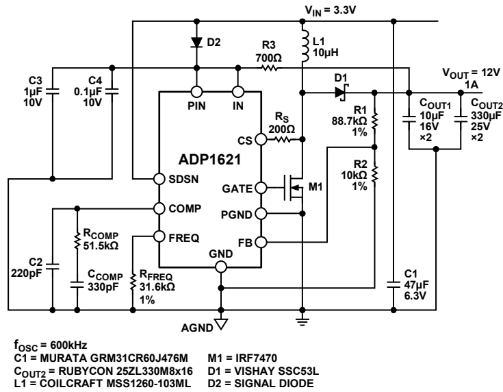
Figure 34. Bootstrapped Application Circuit for V_{OUT} > 5.5\text{ V}
