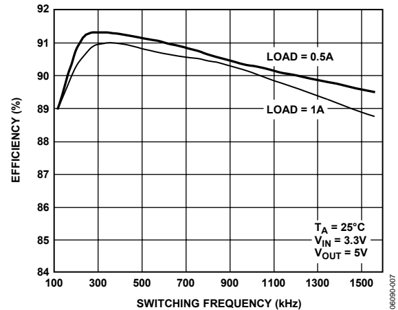
Figure 8. Efficiency vs. Switching Frequency
