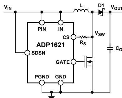
Figure 28. CS Pin Connection for V_{SW} < 30 V, Lossless Mode (No Current-Sense Resistor Needed)
