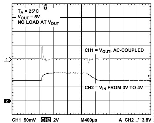
Figure 27. Line Transient Response of the Configuration Shown in Figure 1 with No Load
