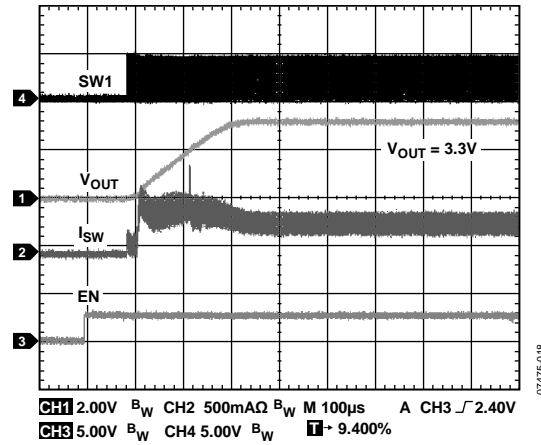
Figure 24. Startup into PWM Mode ( V_{OUT} = 3.3\text{ V} , I_{OUT} = 300\text{ mA} )
