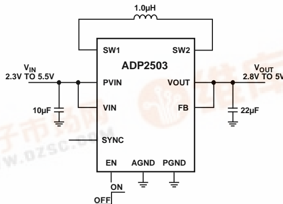
Figure 1. Application Circuit
