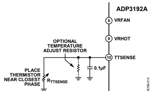
Figure 15. VR Thermal Monitor Circuit
