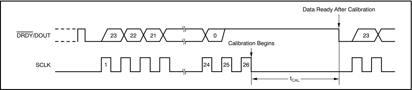
Figure 30. Self-Calibration Timing
