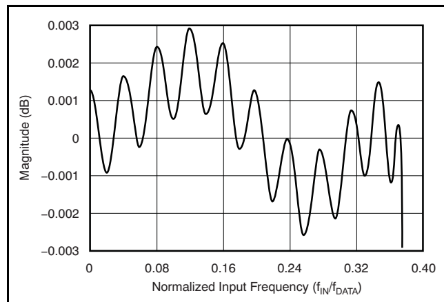
Figure 46. FIR Passband Magnitude Response ( f_{DATA} = 500\text{Hz} )
