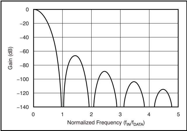
Figure 43. Sinc Filter Frequency Response
