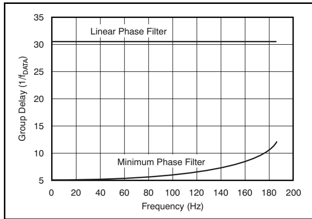
Figure 49. FIR Group Delay ( f_{\text{DATA}} = 500\text{Hz} )
