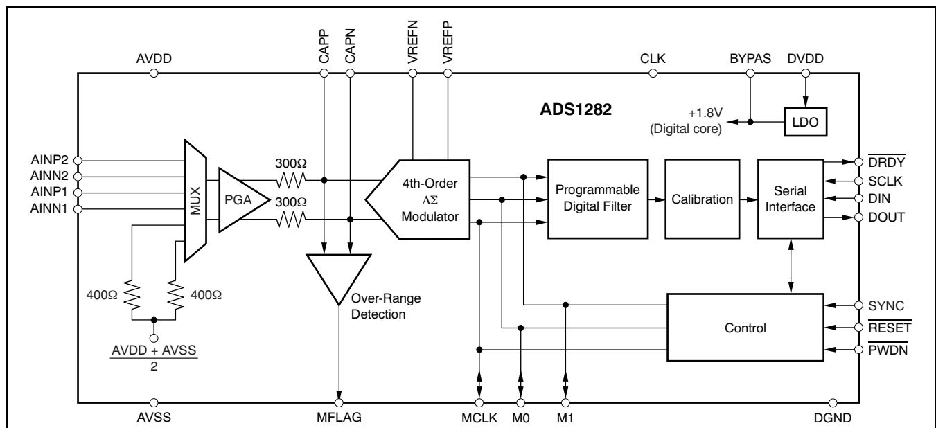
Figure 30. ADS1282 Block Diagram
