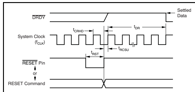
Figure 54. Reset Timing
