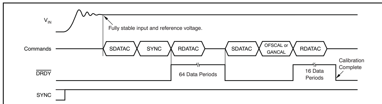
Figure 65. Offset/Gain Calibration Timing
