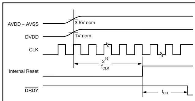
Figure 56. Power-On Sequence
