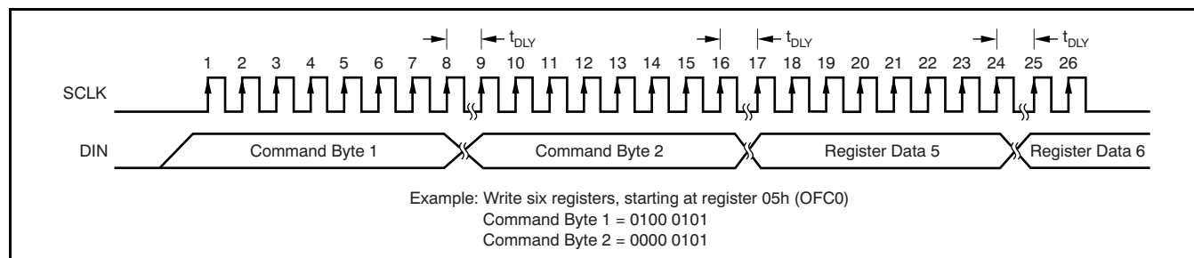
Figure 69. Write Register Data (Table 20 shows t_{DLY} )
