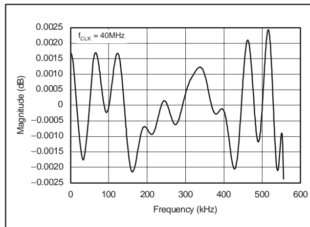
Figure 20. Passband Ripple
