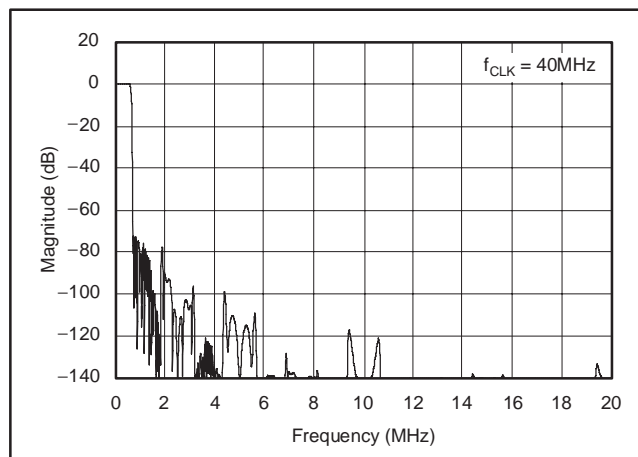
Figure 19. Frequency Response.
