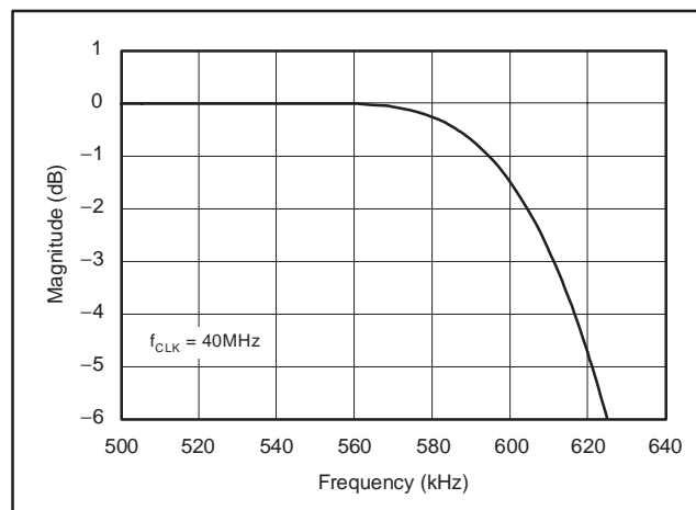
Figure 21. Passband Transition
