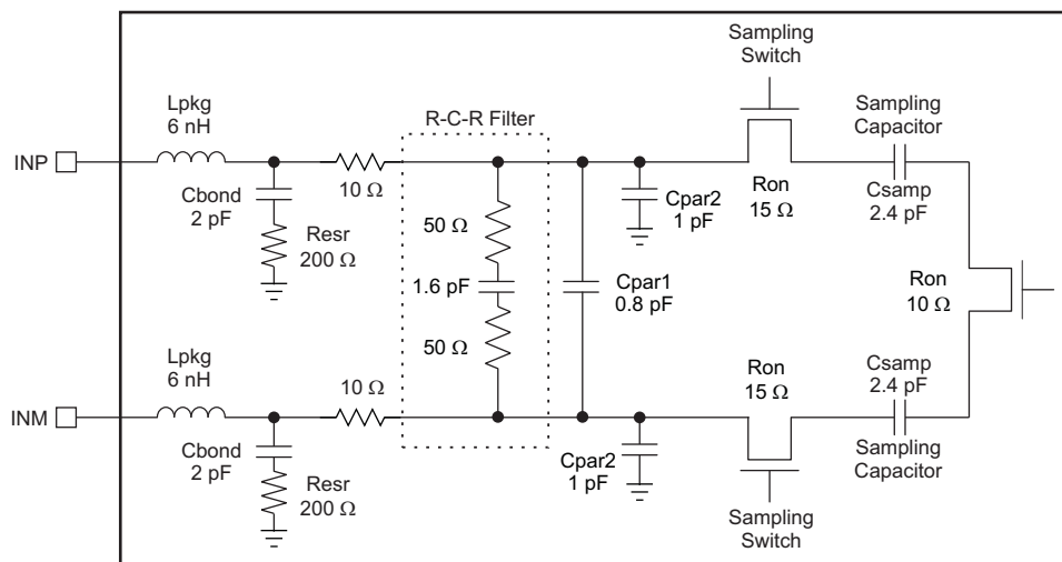
Figure 39. Input Stage
