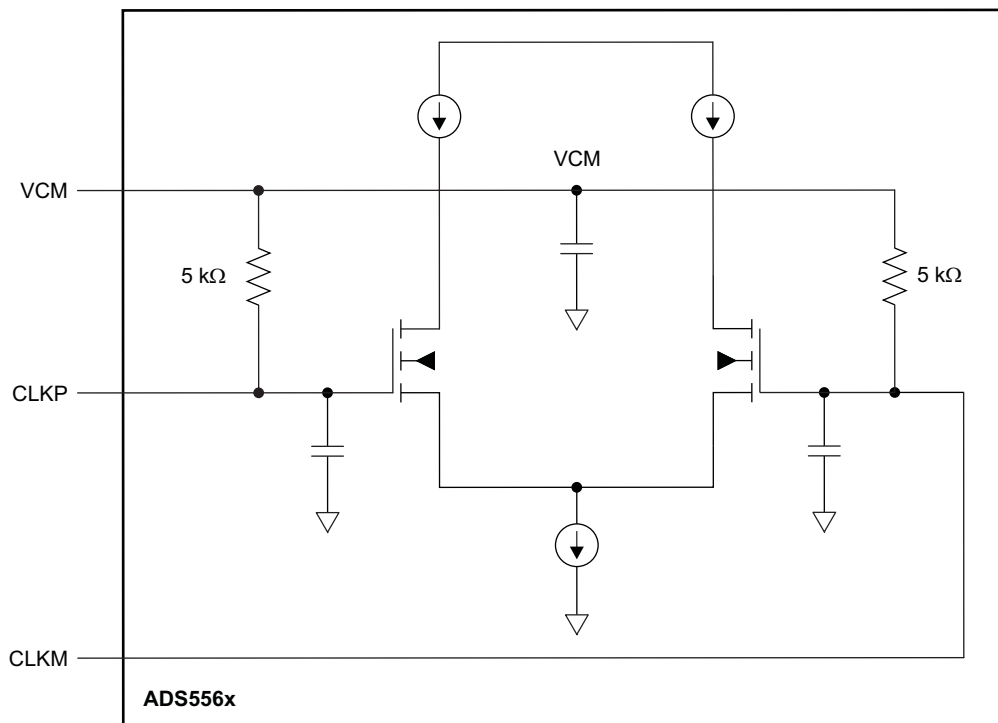
Figure 54. Clock Inputs
