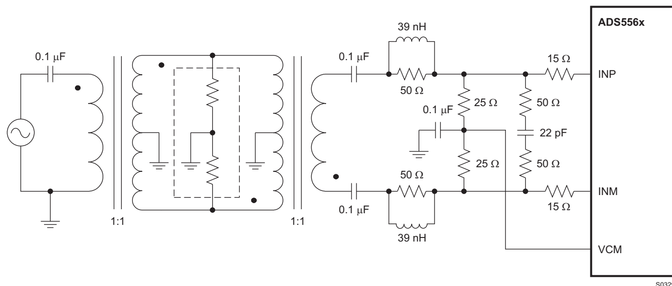
Figure 49. Drive Circuit Using RF transformers
