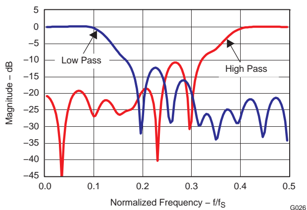
Figure 53. Decimate by 4 Filter Response
