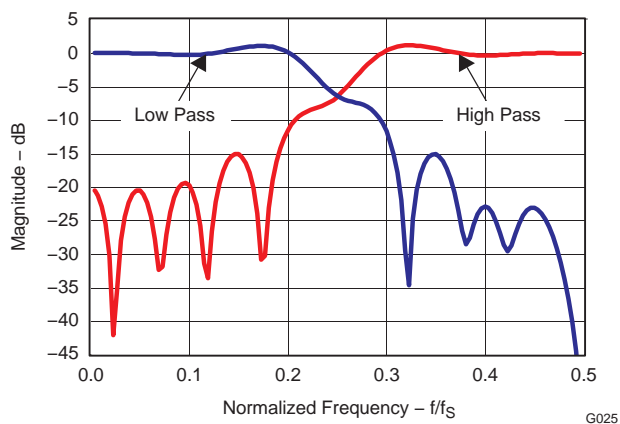
Figure 52. Decimate by 2 Filter Response
