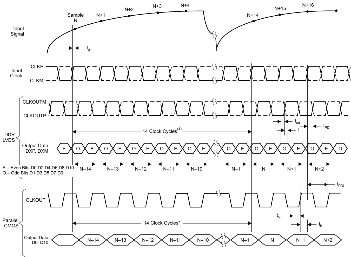
Figure 2. Latency Diagram
