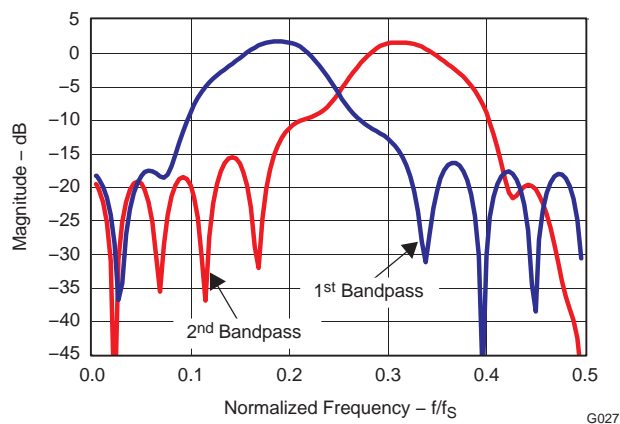
Figure 54. Decimate by 4 Bandpass Response
