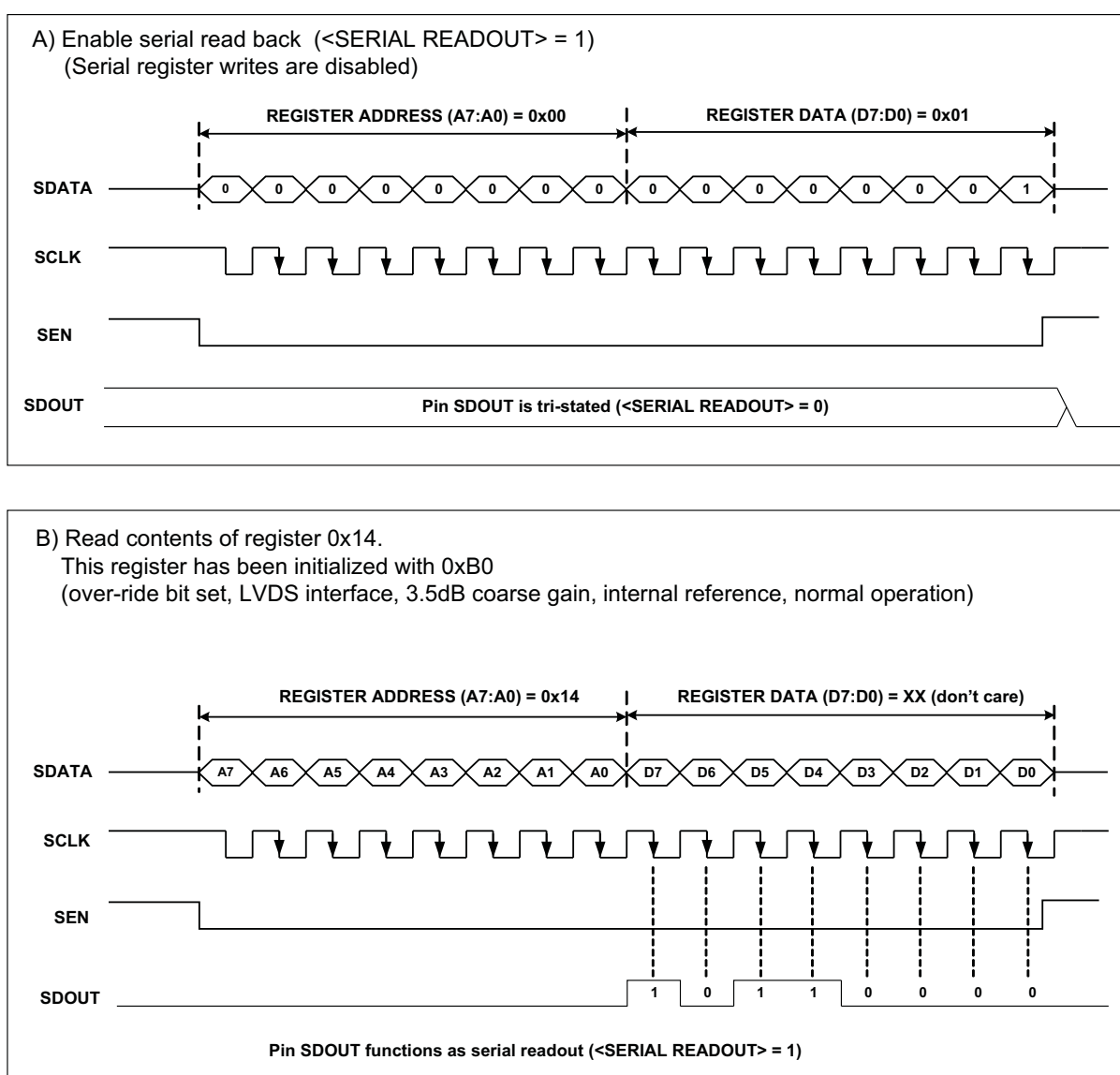
Figure 7. Serial Readout
