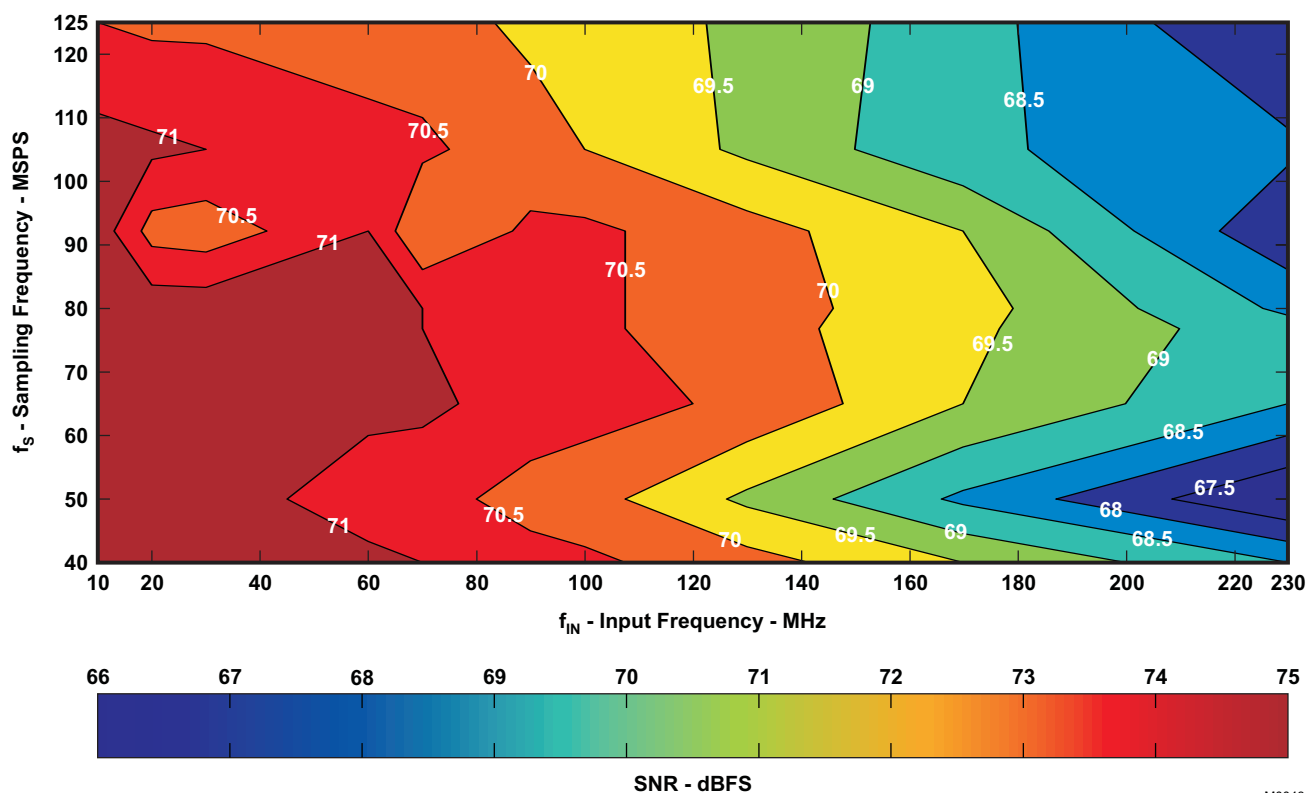
Figure 27. SNR Contour
