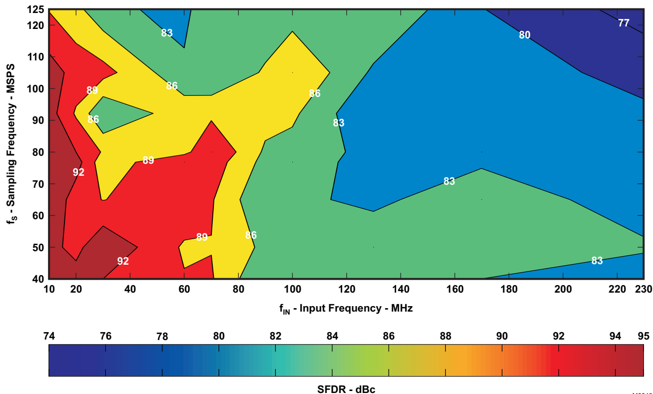
Figure 28. SFDR Contour
