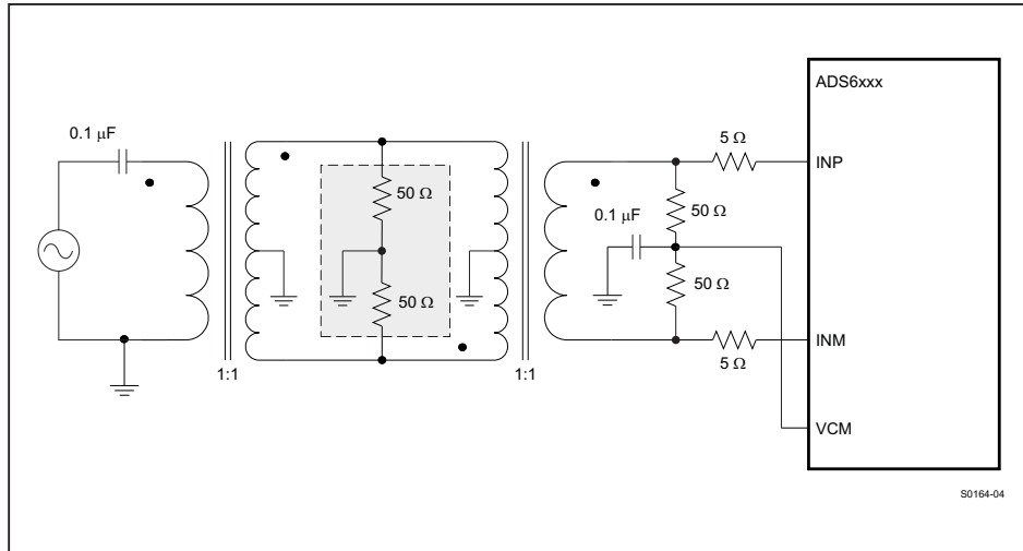
Figure 32. Two Transformer Drive Circuit
