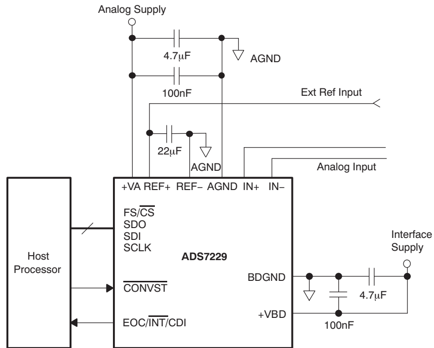
Figure 67. Typical Circuit Configuration
