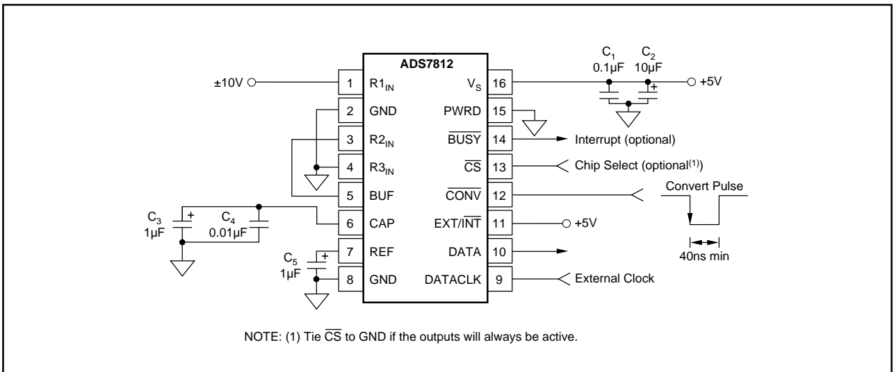
FIGURE 1b. Basic Operation, \pm 10V Input Range, External DATACLK.
