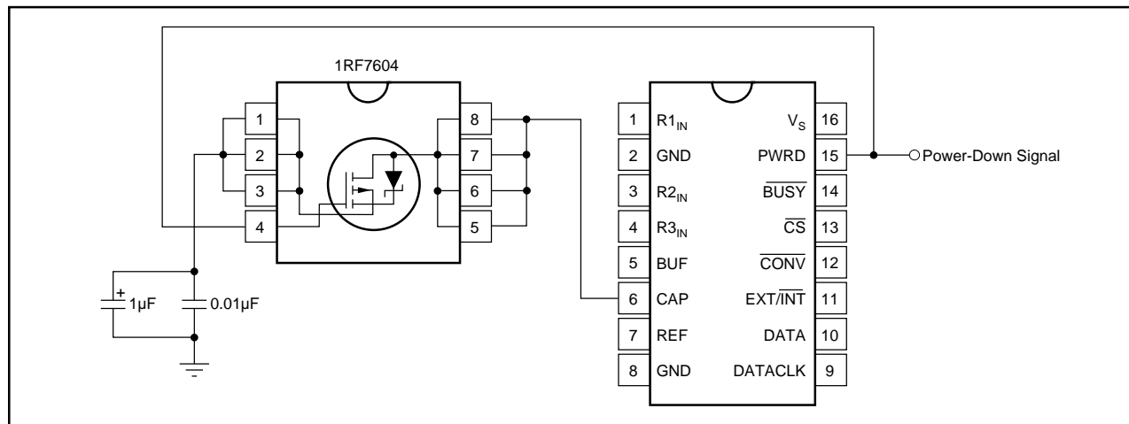
FIGURE 12. Improved Power-Up Response Circuit.
