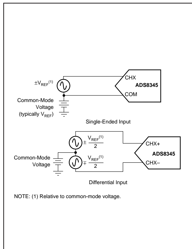
FIGURE 2. Methods of Driving the ADS8345—Single-Ended or Differential.
