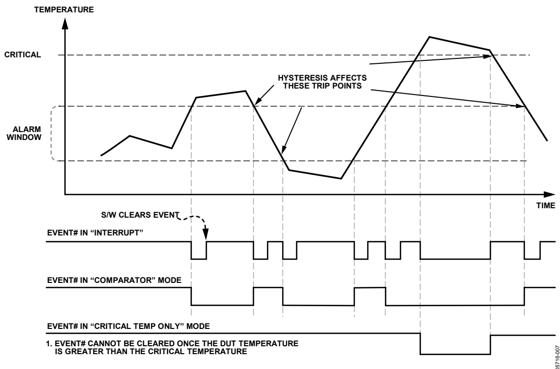
Figure 12. Temperature, Trip, and Events
