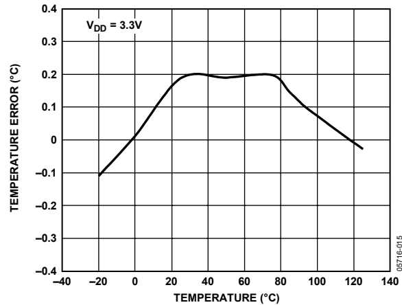
Figure 5. Temperature Accuracy
