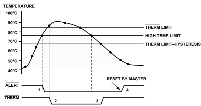
Figure 82. \overline{\text{THERM}} Behavior
