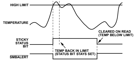
Figure 39. \overline{\text{ALERT}} and Status Bit Behavior
