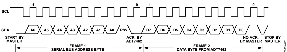
Figure 27. Reading Data from a Previously Selected Register
