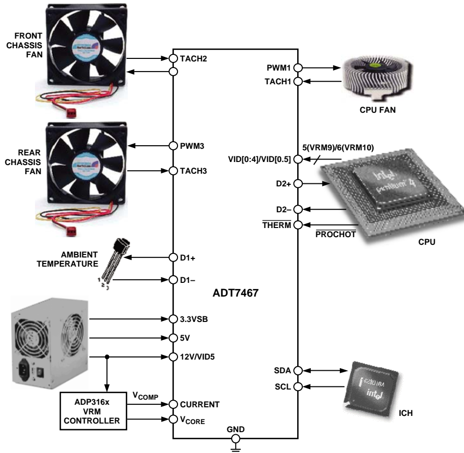
Figure 52. Recommended Implementation 2
