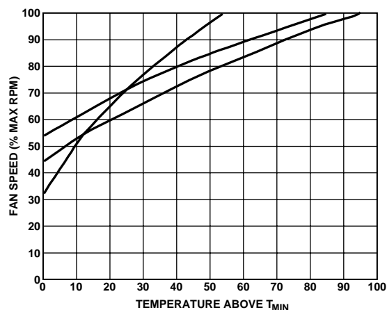
Figure 64. T RANGE and % Fan Speed Slopes for VRM, Ambient, and CPU Temperature Channels
