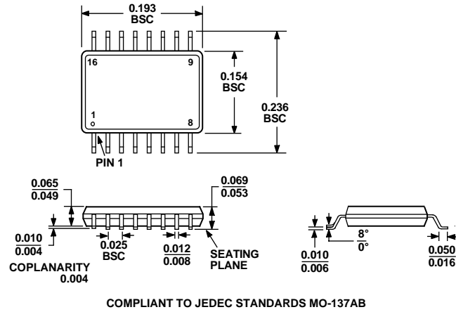
Figure 86. 16-Lead Shrink Small Outline Package [QSOP] (RQ-16) Dimensions shown in inches
