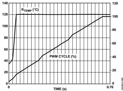
Figure 80. Enhanced Acoustics Mode with Ramp Rate = 48
