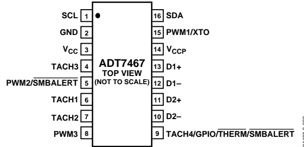
Figure 3. Pin Configuration
