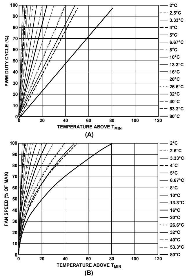
Figure 58. T_{\text{RANGE}} vs. Actual Fan Speed (Not PWM Drive) Profile
