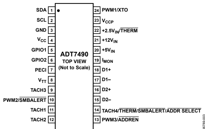
Figure 3. Pin Configuration
