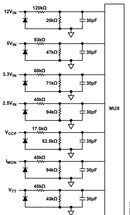
Figure 25. Analog Inputs structure
