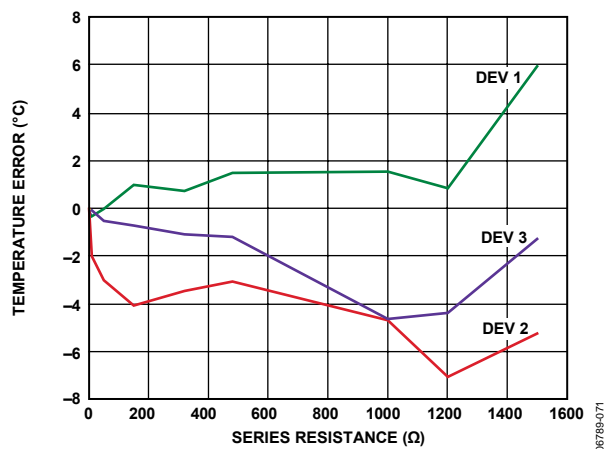
Figure 10. Temperature Error vs. Series Resistance
