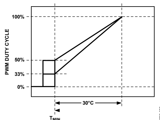
Figure 55. Adjusting PWM MIN Changes the Automatic Fan Control Slope
