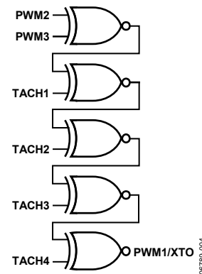
Figure 62. XNOR Tree Test
