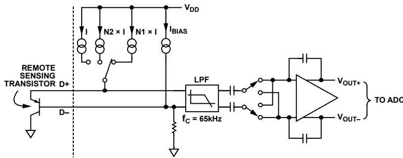
Figure 28. Signal Conditioning for Remote Diode Temperature Sensors
