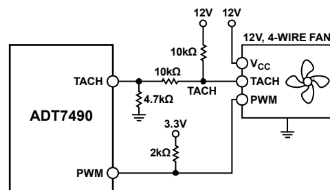
Figure 39. Driving a 4-Wire Fan
