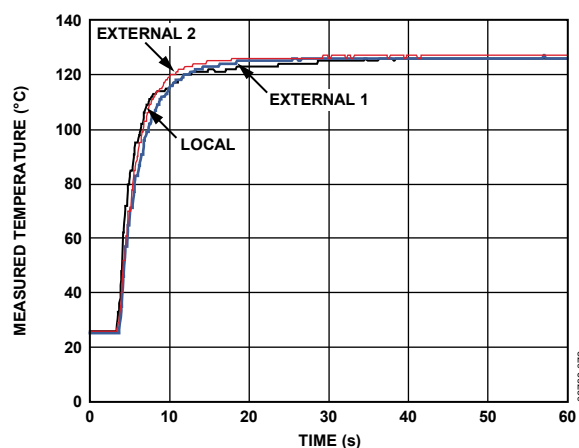
Figure 9. ADT7490 Response to Thermal Shock
