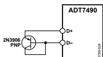
Figure 27. Measuring Temperature Using a PNP Transistor
