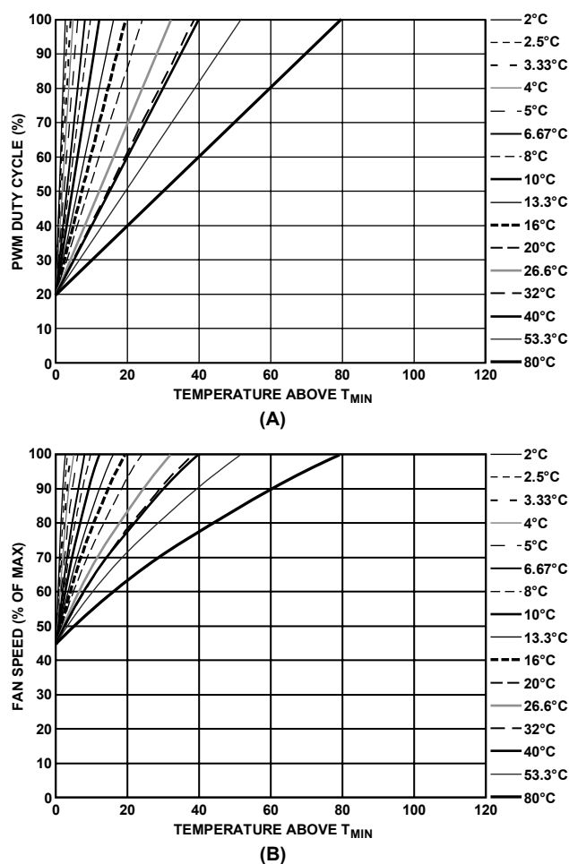
Figure 59. T_{\text{RANGE}} and % Fan Speed Slopes with \text{PWM}_{\text{MIN}} = 20\%
