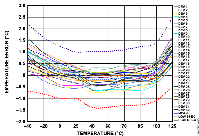
Figure 7. Remote 1 Temperature Sensor Error
