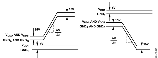
Figure 11. Common-Mode Transient Immunity Waveforms, Input to Output
