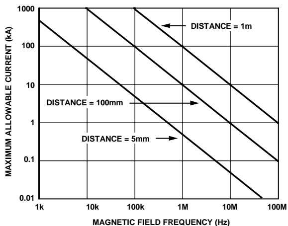
Figure 12. Maximum Allowable Current for Various Current-to-ADuM1310 Spacings
