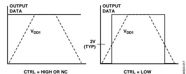
Figure 13. V_{DD1} Power-Up/Power-Down Characteristics, Input Data = High
