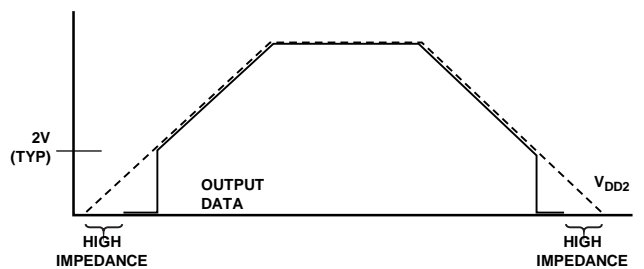
Figure 15. V_{DD2} Power-Up/Power-Down Characteristics, Input Data = High
