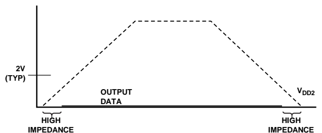
Figure 16. V_{DD2} Power-Up/Power-Down Characteristics, Input Data = Low
