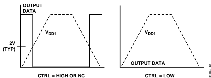
Figure 14. V_{DD1} Power-Up/Power-Down Characteristics, Input Data = Low
