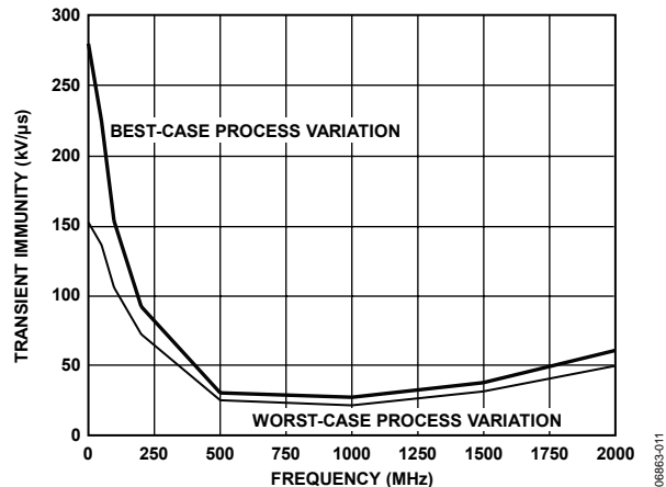
Figure 11. Transient Immunity (Sinusoidal Transients), 27°C Ambient Temperature
