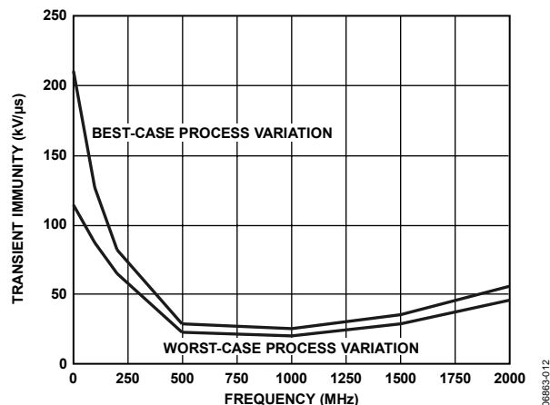
Figure 12. Transient Immunity (Sinusoidal Transients), 100°C Ambient Temperature
