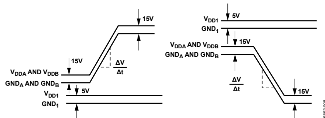
Figure 8. Common-Mode Transient Immunity Waveforms, Input to Output
