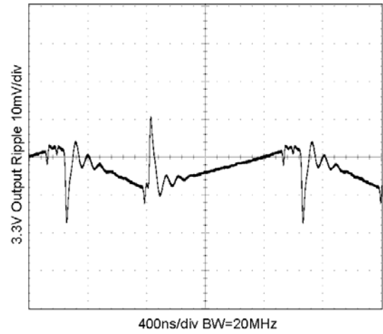
Figure 10. Typical V_{iso}=3.3V Output Voltage Ripple at 90% Load
