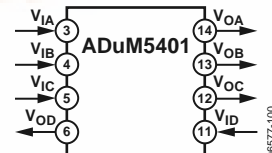
Figure 2. ADuM5401
