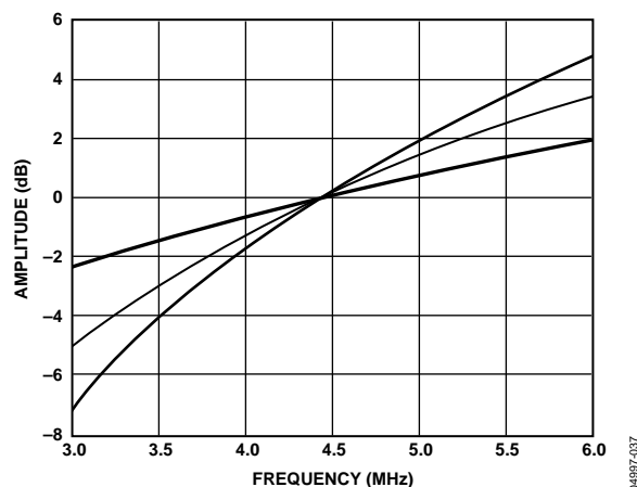
Figure 37. PAL IF Compensation Filter Responses
