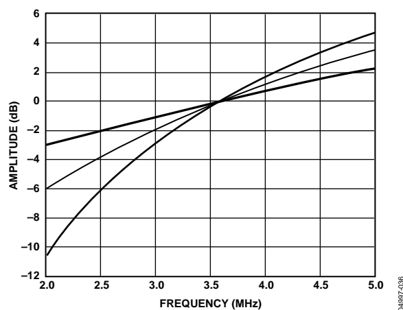
Figure 36. NTSC IF Compensation Filter Responses
