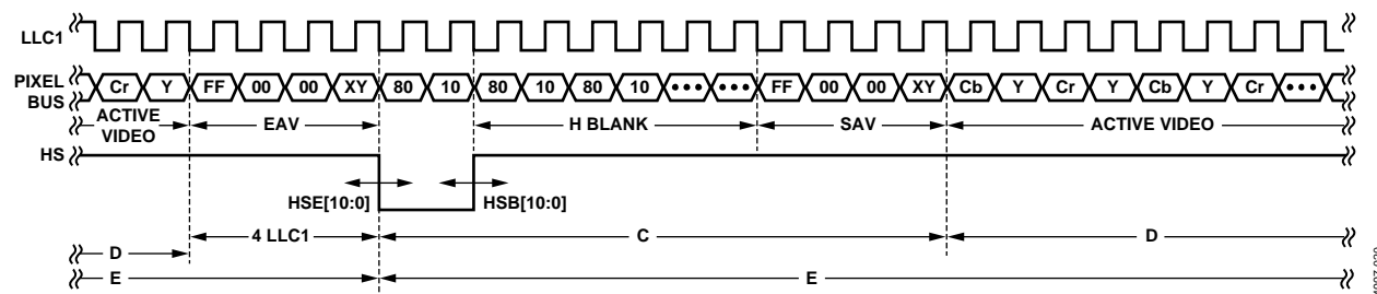
Figure 20. HS Timing
