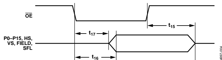
Figure 4. OE Timing
