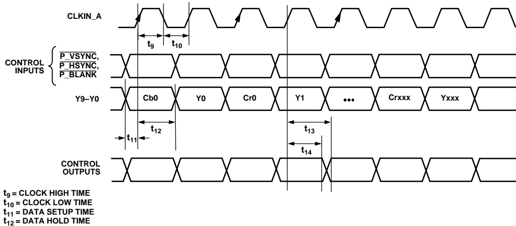
Figure 7. PS 4:2:2 10-Bit Interleaved at 54 MHz HSYNC/VSYNC Input Mode (Input Mode 111)
