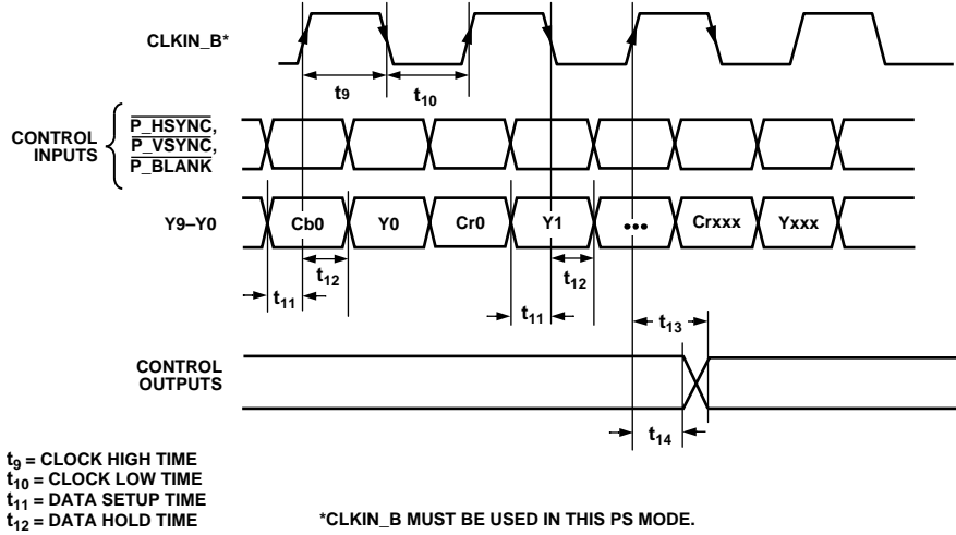
Figure 6. PS 4:2:2 10-Bit Interleaved at 27 MHz HSYNC/VSYNC Input Mode (Input Mode 100)
