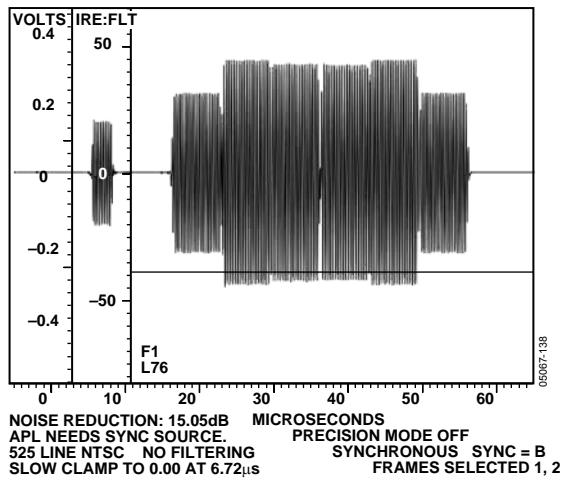
Figure 138. NTSC Chroma
