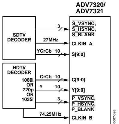
Figure 52. Simultaneous HD and SD Input
