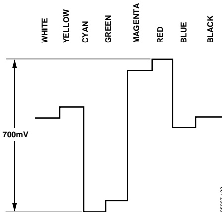
Figure 132. Pb Levels—PAL
