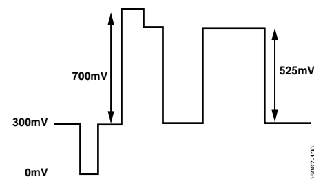
Figure 130. SD RGB Output Levels—RGB Sync Enabled
