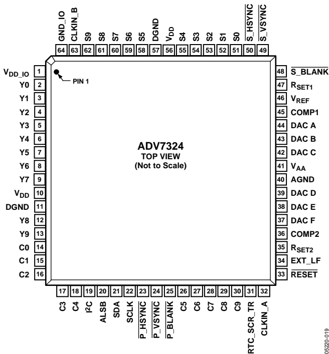
Figure 19. Pin Configuration
