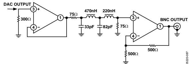
Figure 87. Example of Output Filter for HDTV, 2x Oversampling
