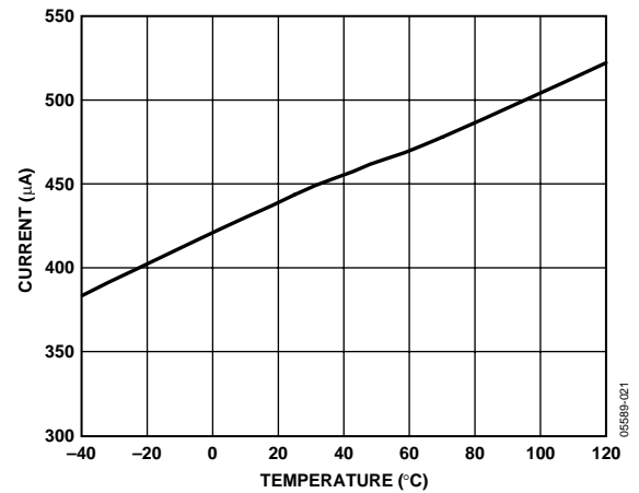
Figure 21. Supply Current vs. Temperature V_s=3V
