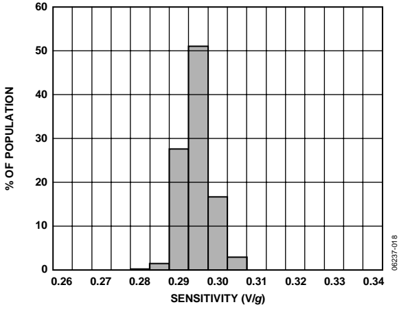
Figure 18. X-Axis Sensitivity at 25°C, V_s = 3 V
