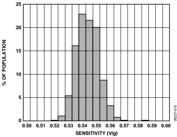
Figure 19. X-Axis Sensitivity at 25°C, V_s = 5 V
