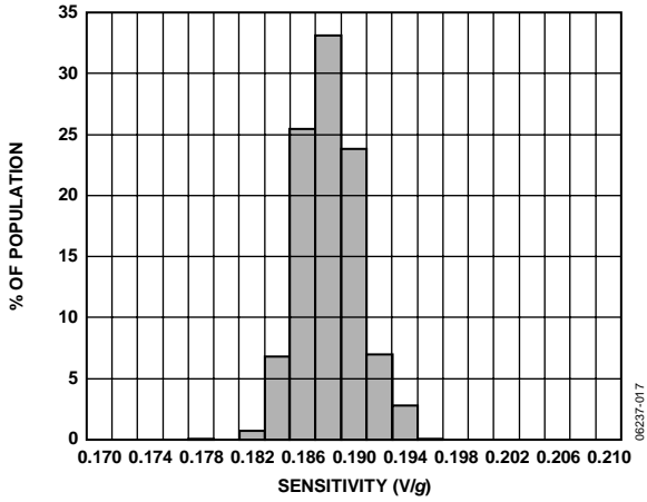
Figure 17. X-Axis Sensitivity at 25°C, V_s = 2 V
