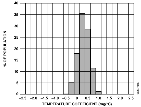
Figure 15. Y-Axis Zero g Bias Temperature Coefficient, V_S = 5\text{ V}
