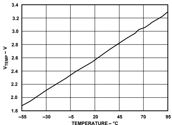
Figure 5. Temperature Sensor Output
